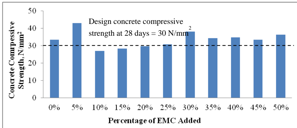
Fig. 6. Relationship between 28-days concrete compressive strength and percentage of EMC added
