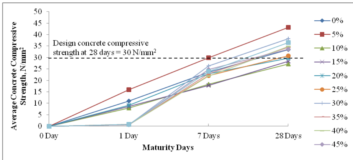
Fig. 3. Relationship between the average concrete compressive strength and maturity days
