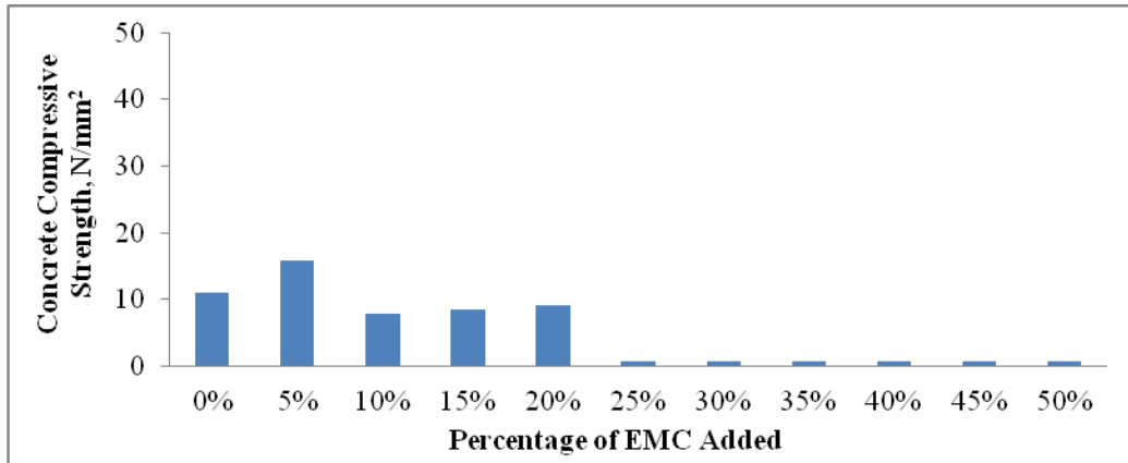
Fig. 4. Relationship between 1-day concrete compressive strength and percentage of EMC added
