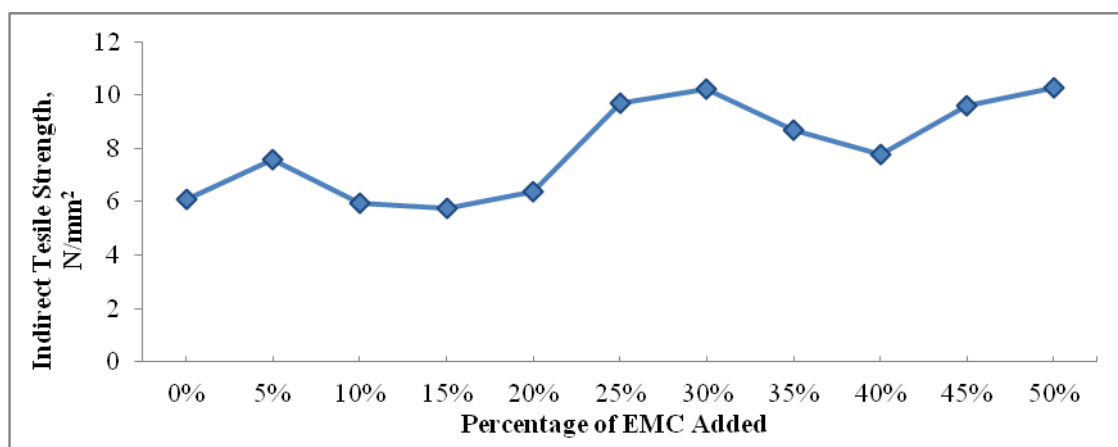
Fig. 7. Relationship between indirect tensile strength and percentage of EMC added
