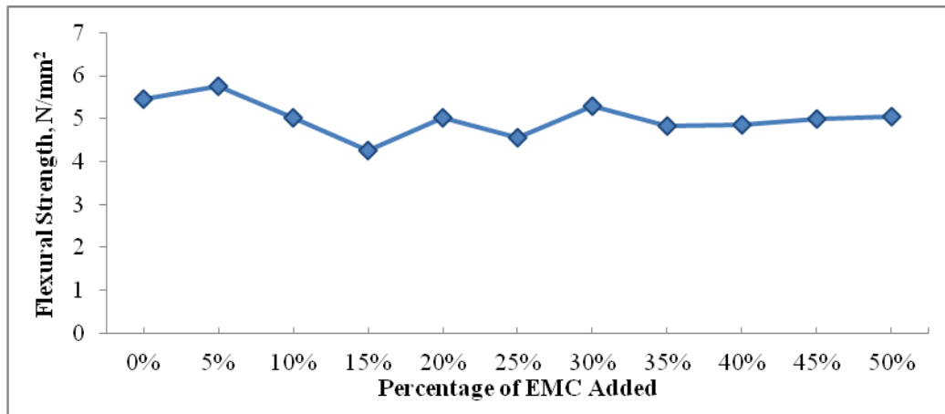
Fig. 8. Relationship between flexural strength and added percentage of EMC
